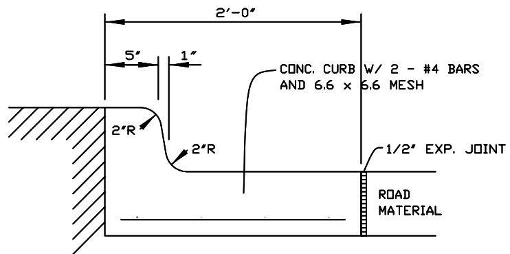
CURB SECTION
